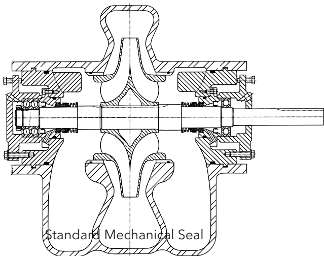
Mechanical Seal Mounted on shaft
